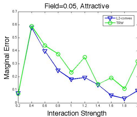
Fig. 5. Comparison of error in marginal probabilities on a complete graph, estimated by tree-reweighted free energy approximation and L_2 convex free energy approximation. The graphs present the average error over 100 random trials
